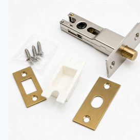
WK-103 60mm Square Bolt Latch
