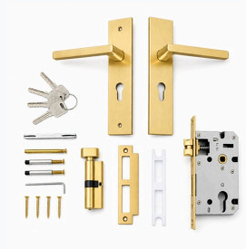
WK-204 Brass Mortise Lock
